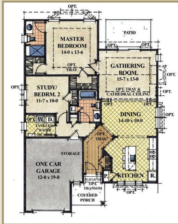
Main Floor - 1,254 sq.ft.
