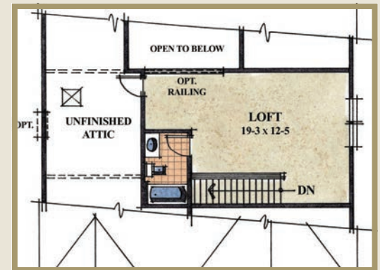
Second Floor Option 2 - 430 sq.ft.
