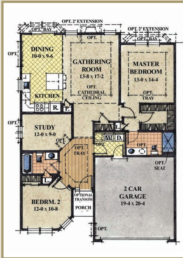
Main Floor - 1,370 sq.ft.
