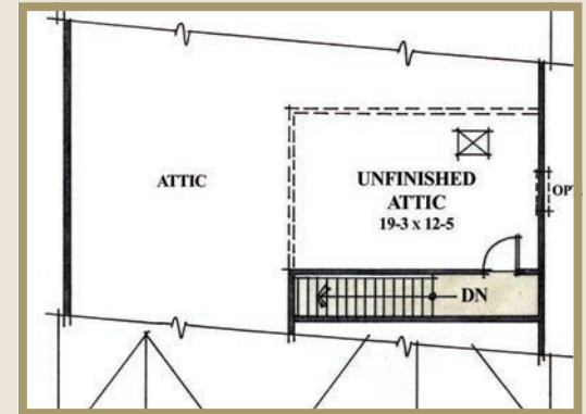
Second Floor Option 1
