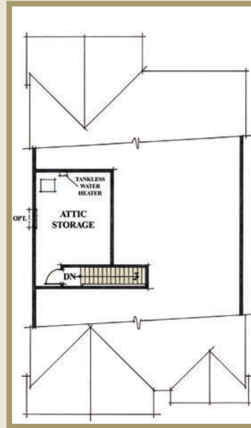
Second Floor Standard
