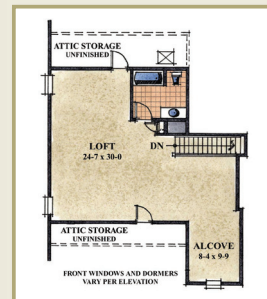
Second Floor Option 1 - 741 sq.ft.
