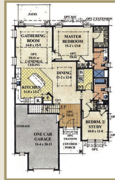
Main Floor Option 2 1 Car Garage with Second Floor Option
