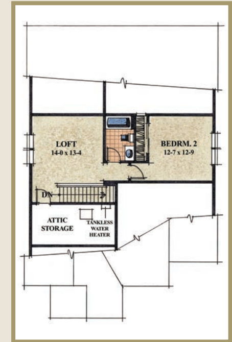
Second Floor Option 3 - 514 sq.ft. Loft/Bath/Bedroom
