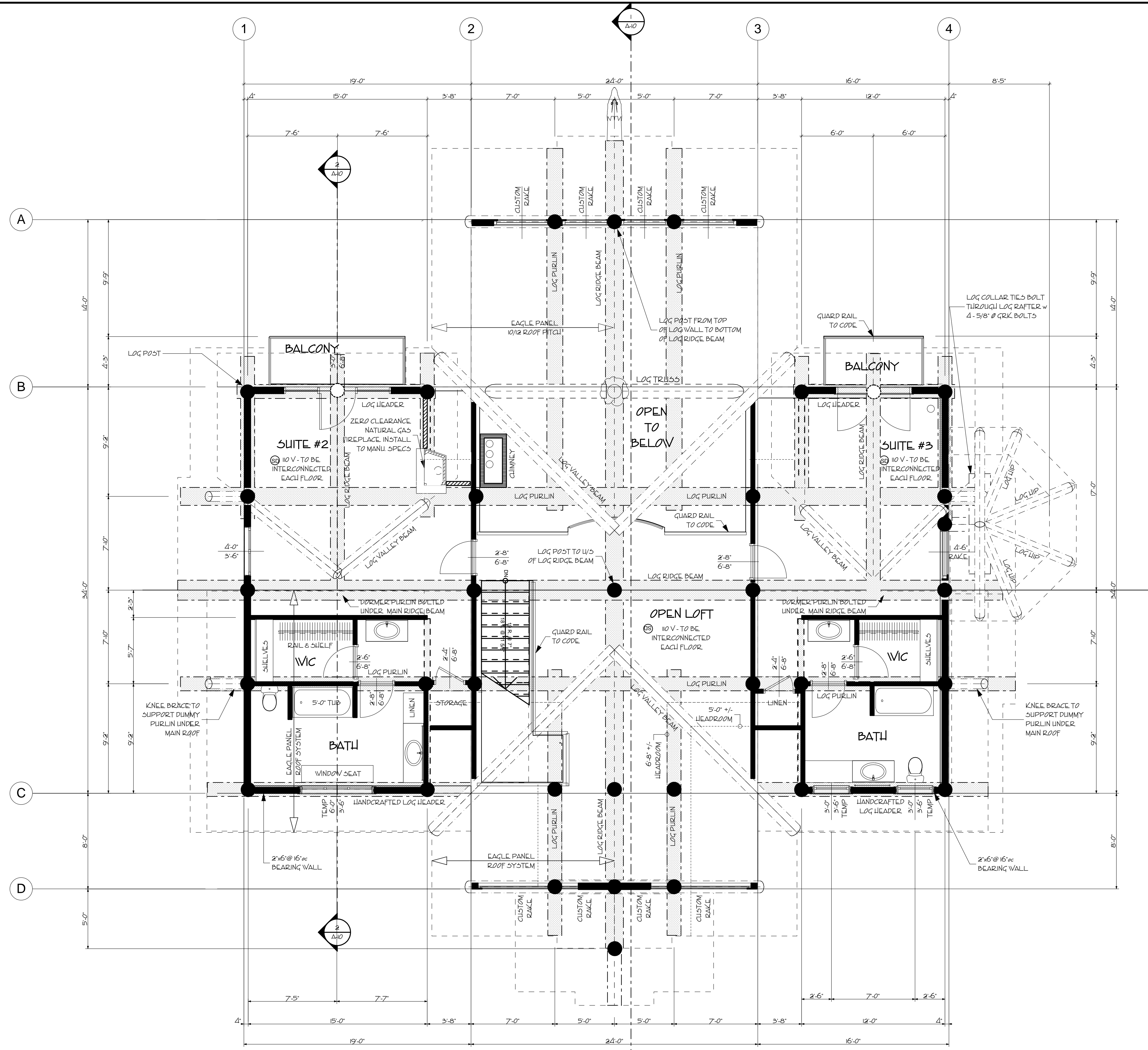
LOFT FLOOR PLAN
