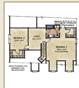
Second Floor Option 3 - 972 sq.ft.
