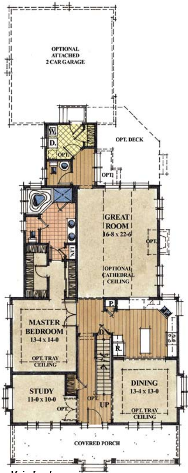
Main Level Standard Elevation & Elevation 2 - 1,706 sq.ft.
