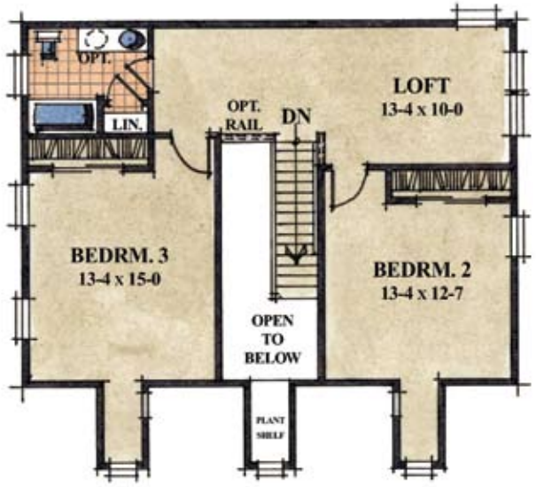
Second Level Standard Elevation - 829 sq.ft.
